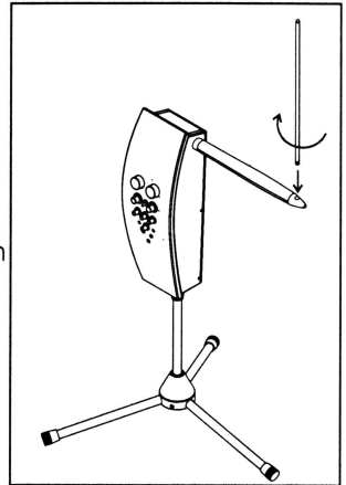
Figure 9 - installing the Pitch Antenna
